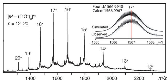
Figure 2. CSI-TOF mass spectrum of complex 2 (TfO − salt), with an inset showing the observed and simulated isotopic patterns of the 17 + signal.
