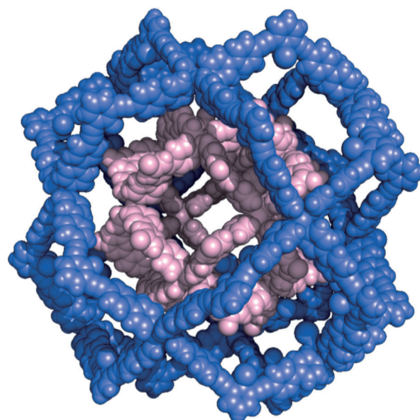
Figure 3. Crystal structure of the sphere-in-sphere complex 2 . All atoms are depicted as sphere models. Atoms of the interior sphere are in pink, and the exterior sphere are in blue. Counterions (TfO − ) and the TEG linkers are omitted for clarity.
