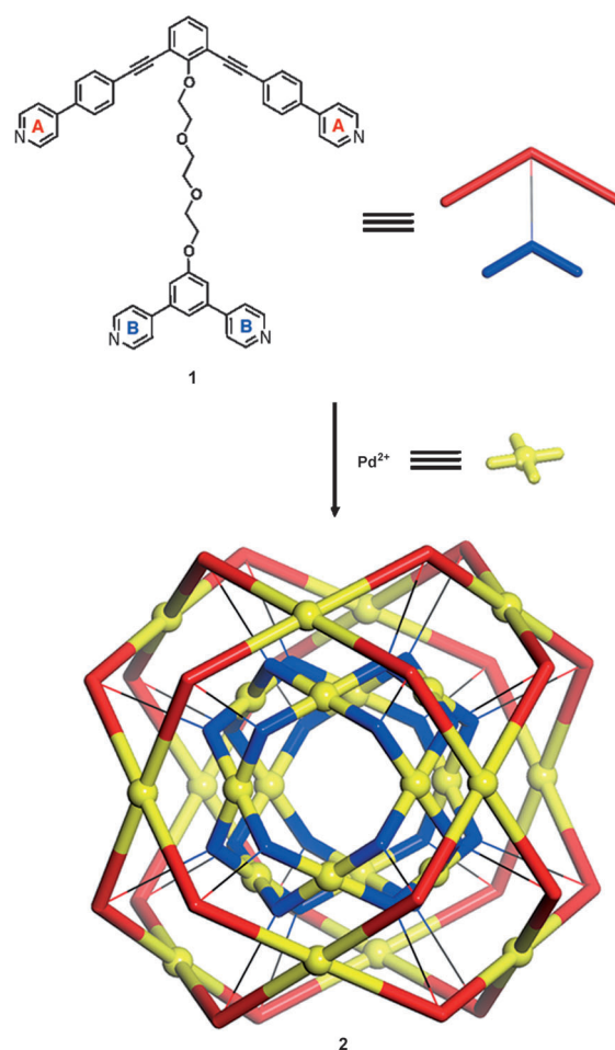
Scheme 1. Self-assembly of sphere-in-sphere complex 2 .
