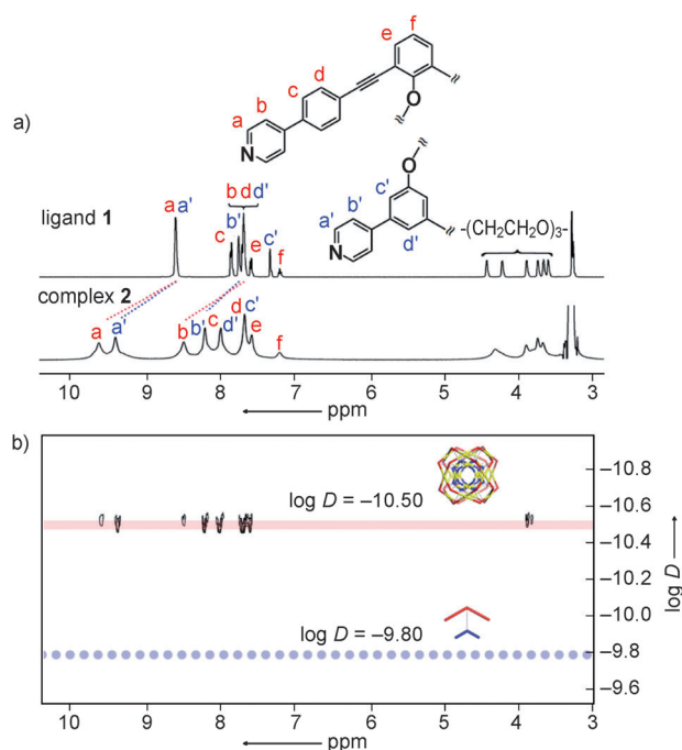
Figure 1. a) 1 H NMR (500 MHz, [D 6 ]DMSO, 300 K) spectra of ligand 1 and complex 2 (NO 3 − salt). b) 1 H DOSY (500 MHz, [D 6 ]DMSO, 300 K) spectrum of complex 2 (the region for ligand 1 is also indicated by a blue dotted line).
